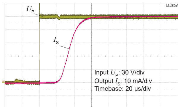
Figure 6: Typical step response (0 to 150 V)
