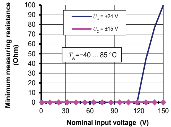
Figure 2: Minimum measuring resistance For T_A under 80 °C, the minimum measuring resistance is 0 \Omega whatever U_C
