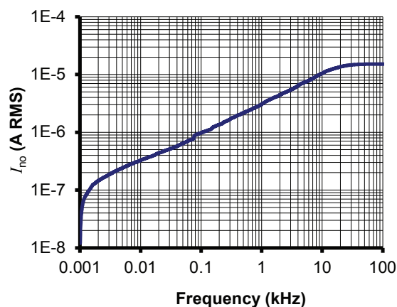
Figure 16: Typical total output RMS noise current with R_M = 50 \Omega ( f_c is upper cut-off frequency of bandpass, low cut off frequency is 1 Hz)
