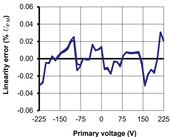
Figure 17: Typical linearity error at 25 °C
